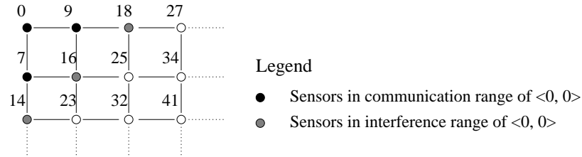
Figure 5.2: Sample diffusion for convergecast where communication range=1, interference range=2. The number associated with each sensor denotes the time at which it forwards the diffusion message.
