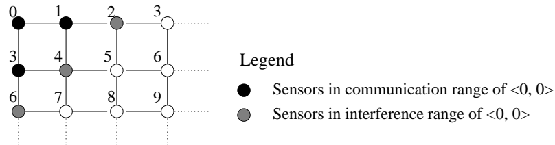
Figure 3.6: Sample diffusion in networks where a sensor communicates with its distance 1 neighbors and interferes with its distance 2 neighbors. The number associated with a sensor shows the slot in which it should transmit.
