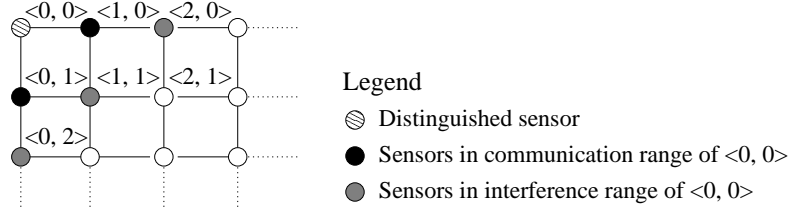
Figure 2.1: Sensor network topology where a sensor communicates with its distance 1 neighbors and interferes with its distance 2 neighbors. The numbers associated with a sensor indicates the grid position of the sensor.
