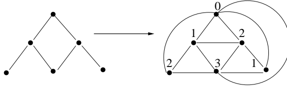
Figure 6.7: Transformation using graph coloring. The number associated with each process denotes the color of the process.
