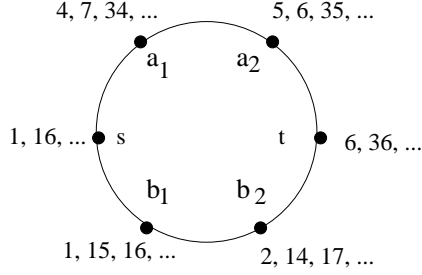
Figure 6.4: Executing more than one process in untimed systems. The numbers associated with each process denotes the number of writes the process executes in the corresponding round.
