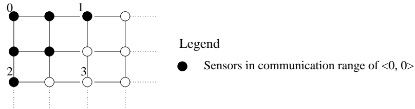
Figure 3.4: Sample diffusion in networks where a sensor communicates with its distance 2 neighbors. The number associated with a sensor shows the slot in which it should transmit.
