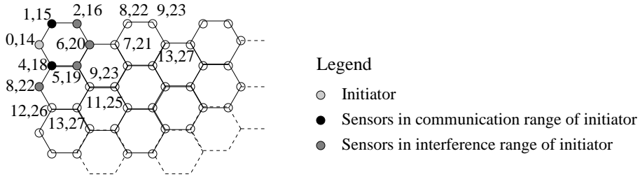
Figure 4.4: TDMA slot assignment in hexagonal-grid network where communication range=1 and interference range=2. The number associated with each sensor denotes the time at which it can send a message. Slots for some sensors are not shown.
